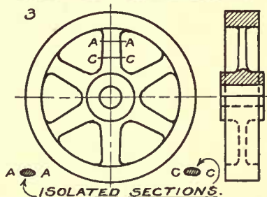
ISOLATED SECTIONS.
